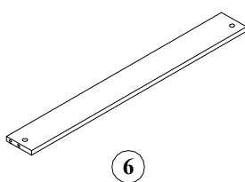
6 # RJ038-010-023-FSRA # RJ038-010-024-FSRA x4 Front Support Rail x4 Rail de support avant x4 Riel de soporte delantero
