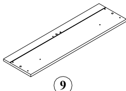
9 # RJ038-010-023-DFPA # RJ038-010-024-DFPA x6 Drawer Front Panel x6 Panneau avant du tiroir x6 Panel frontal del cajón
